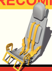
Q72361 Heinkel He 162A Ejection Seat
